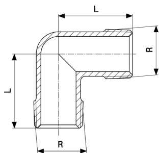
Koleno 90° - mosadz model 1611
